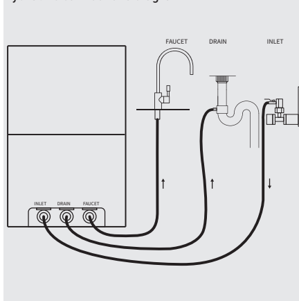
Hydraulic connections diagram Hydraulic connections diagram
