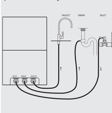
Hydraulic connections diagram
